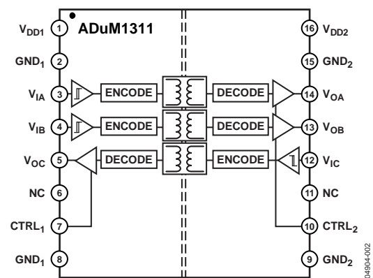
Figure 2. ADuM1311
